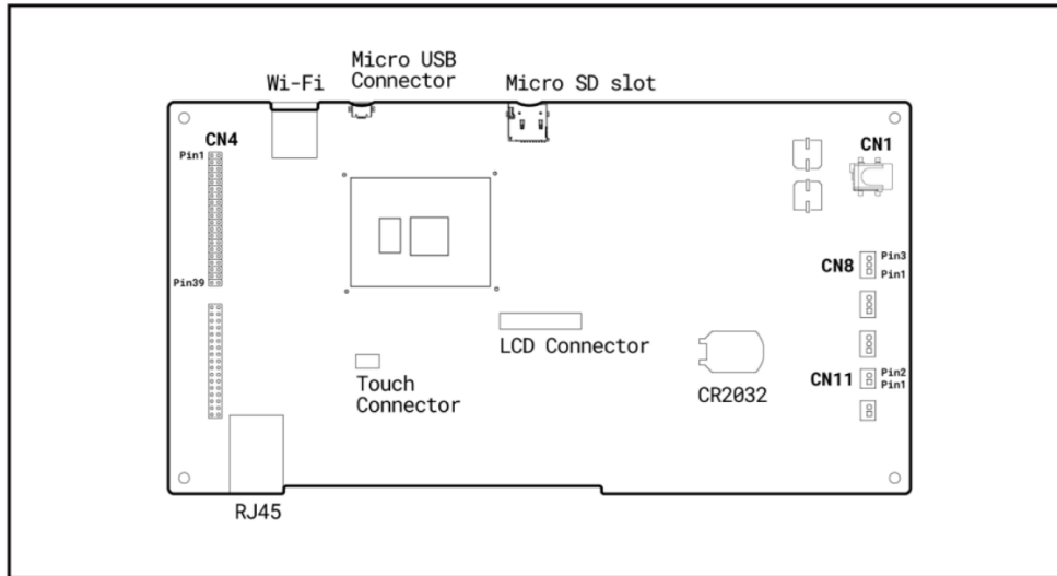
Figure 1. Control Board Outline
