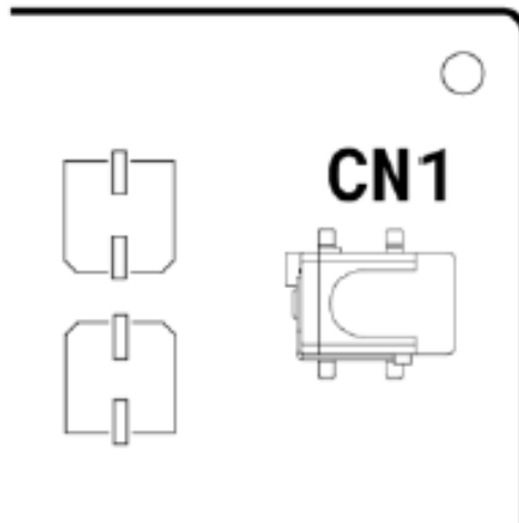
Figure 5. CN1 Pin Definition
