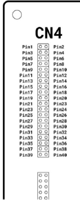
Figure 2. CN4 Pin Definition
